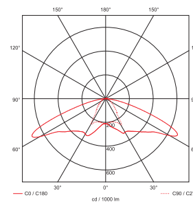
optika 60°x120° 4000K
