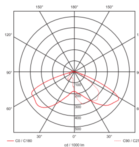
optika 70°x140° 4000K
